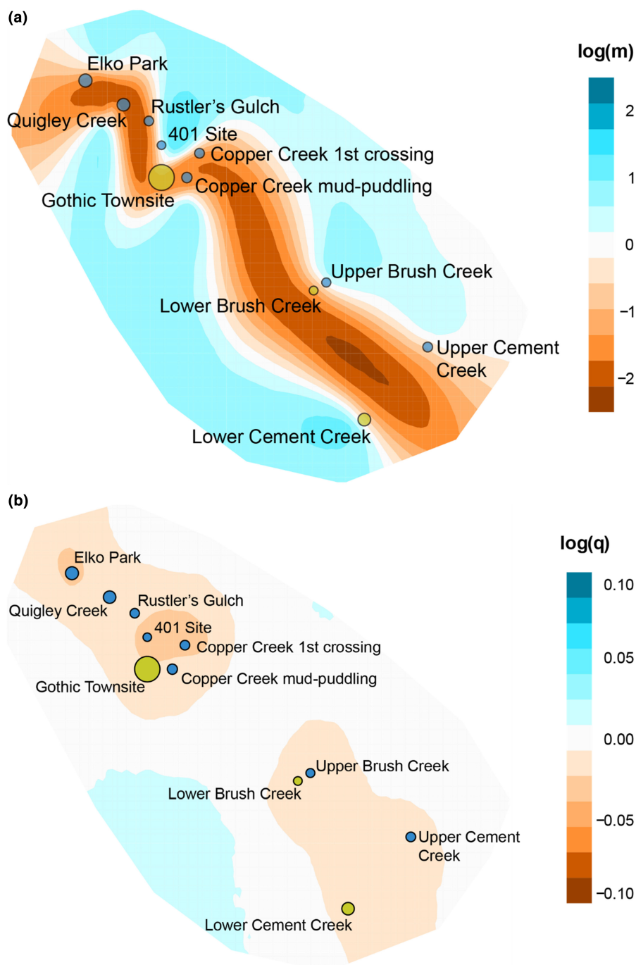
FIGURE 7 (a) Estimated effective migration surfaces and (b) Estimated effective diversity surfaces for P. macdunnoughii in the East River Valley. The migration and diversity rates, \log(m) and \log(q) represent gene flow or genetic diversity barriers and corridors in the habitat respectively. Each value corresponds to a 10-fold increase (blue) or decrease (orange/brown) in migration or genetic diversity compared to the null hypothesis of isolation by distance (white). Sites in blue represent areas where Thlaspi arvense does not occur and sites in yellow represent areas where T. arvense is present.
