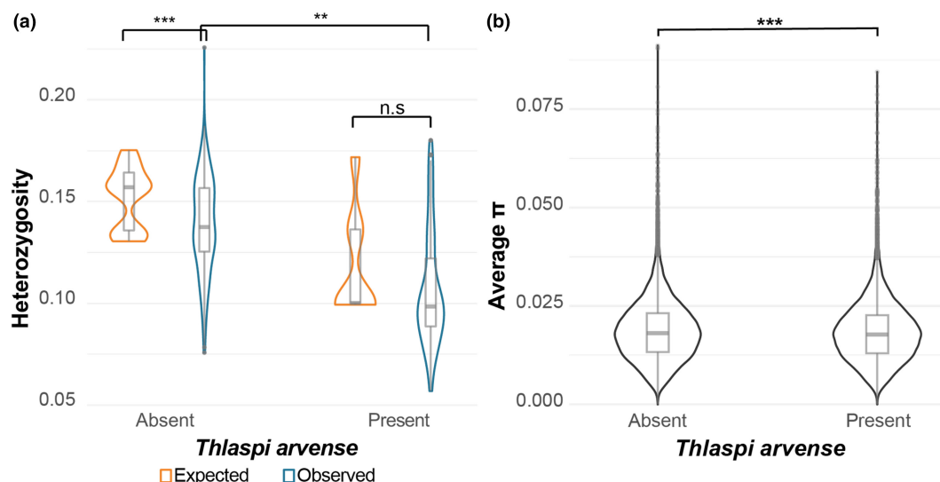
FIGURE 5 (a) Genome-wide variance in expected and observed heterozygosity of P. macdunnoughii in the East River valley. Bartlett's tests were used to compare observed heterozygosity between habitats where T. arvense was present or absent, and observed versus expected heterozygosity within each of these habitat types. (b) Genome-wide variance in nucleotide diversity ( \pi ) of P. macdunnoughii in habitats without and with T. arvense (Bartlett's test, *** p < .001 ).
