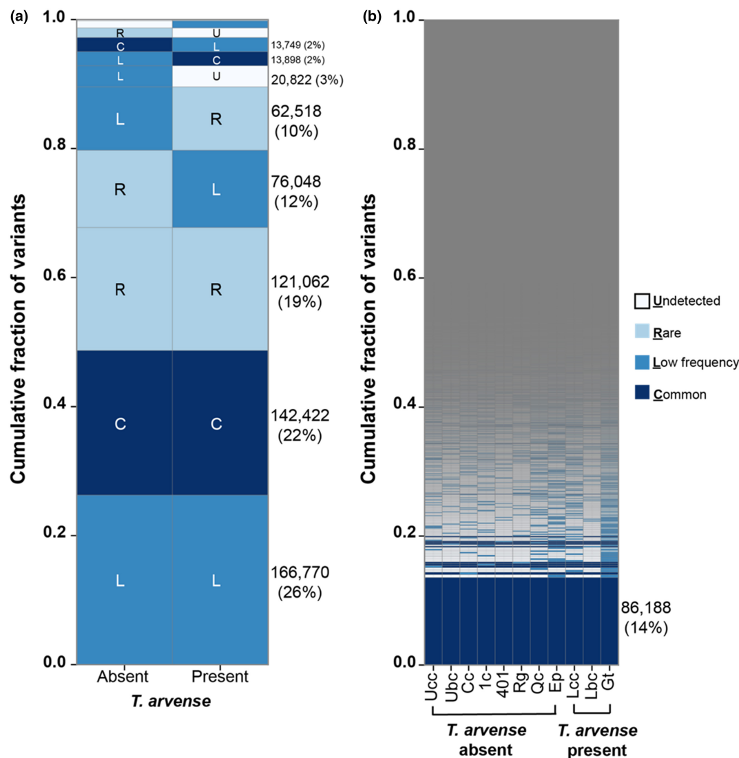
FIGURE 4 (a) Relative abundance of allele frequency variants of P. macdunnoughii in areas with T. arvense and areas without T. arvense . The letters depicted in the figure represent the frequency of the minor allele in the habitat (U-undetected: No alleles present, R-rare: <1% minor allele frequency (MAF), L-low frequency: 1%–5% MAF, C-common: >5% MAF). The percentages and their corresponding numbers indicate the number of variants in each class and are grouped based on SNP identity. (b) Relative abundance of allele frequency variants of P. macdunnoughii in our study area. 1c, 1st Crossing; 401, 401 site; Cc, Copper Creek; p, Elko Park; Gt, Gothic townsite; Lbc, Lower Brush Creek; Lcc, Lower Cement Creek; Qc, Quigley Creek; Rg, Rustler's Gulch; Ubc, Upper Brush Creek; Ucc, Upper Cement Creek. Greyed area represent alleles whose contribution was not significant to the differences between comparisons.
