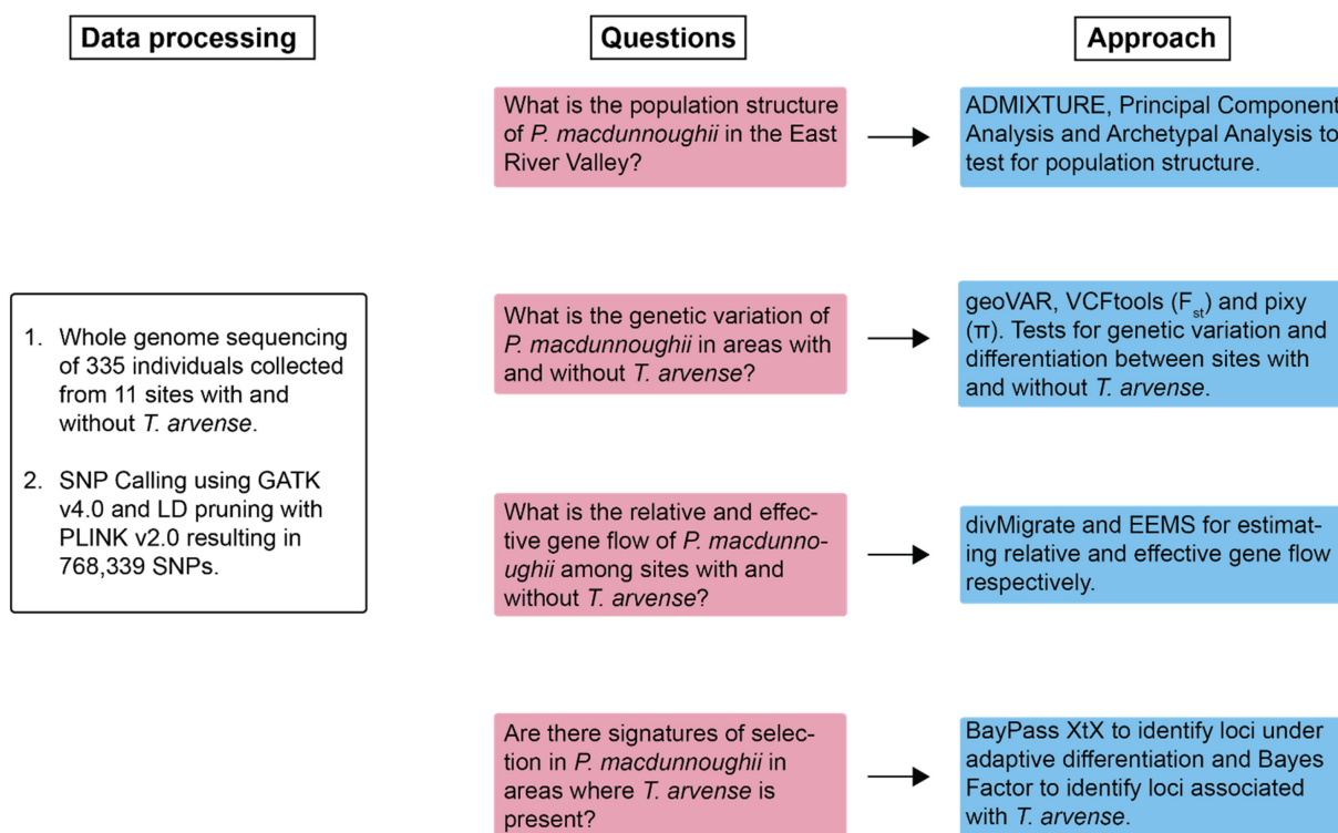
FIGURE 2 Outline of bioinformatic pipelines employed in the analysis of whole-genome sequences of Pieris macdunnoughii to dissect signatures of selection in response to Thlaspi arvense .
