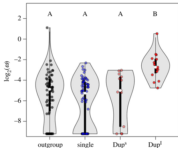
Figure 6. The distributions of omega (dN/dS) estimates for ATP \alpha 1 of non-specialists (outgroup), Apocynaceae-specialists with a single copy of ATP \alpha 1 (single), and specialists with duplicated ATP \alpha 1, where the relatively cardenolide sensitive and insensitive copies are noted as Dup s and Dup l , respectively. The median omega values are indicated with an open circle and bars represent 50% quantiles. There is a significant difference between the omega distributions for Dup l and those of all three other groups (letters A and B indicate significantly different categories; Dup l versus outgroup p = 2 \times 10^{-5} , Dup l versus single p = 3 \times 10^{-7} , Dup l versus Dup s p = 3 \times 10^{-3} ). p -values were estimated using Dunn's test of multiple comparisons using rank sums as implement in R (dunn.test) and adjusted using the Benjamini–Hochberg method.
