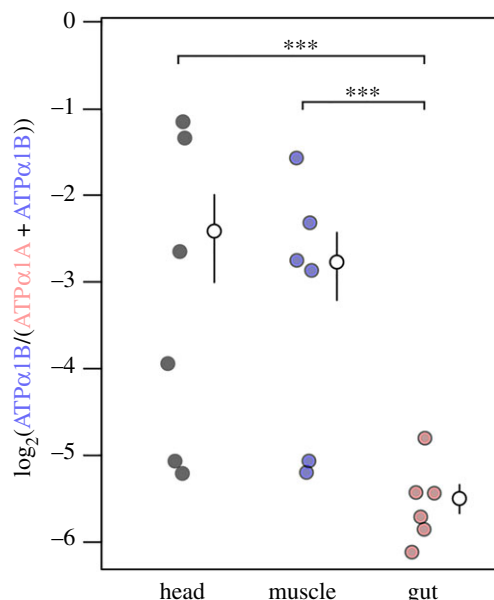
Figure 4. RNAseq-based estimates of ATPα1 expression by tissue in the duplication-bearing Orthopteran Poecilothera pictus . As observed in other Apocynaceae-specialists [29], the relatively more cardenolide-sensitive ATPα1B is significantly less expressed in the gut than in head (corrected p = 8 \times 10^{-4} ) and muscle (corrected p = 9 \times 10^{-4} ) in P. pictus (electronic supplementary material, table S3). The mean proportion of ATPα1B of total ATPα1 is indicated with open circles with two standard errors as whiskers. p -values were estimated using the ‘inverted beta-binomial’ test for paired sample count data (see Methods) *** p < 0.001 .
